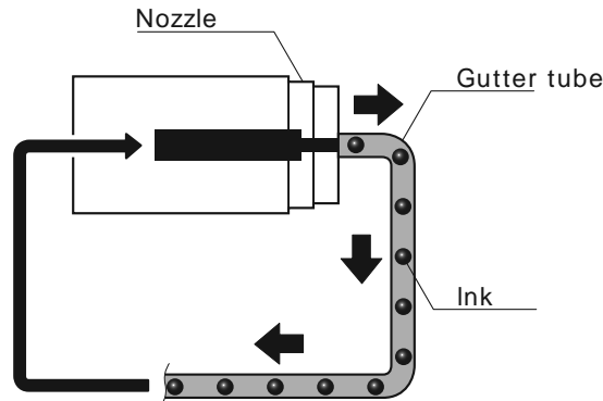
Nozzle sealed with the gutter
